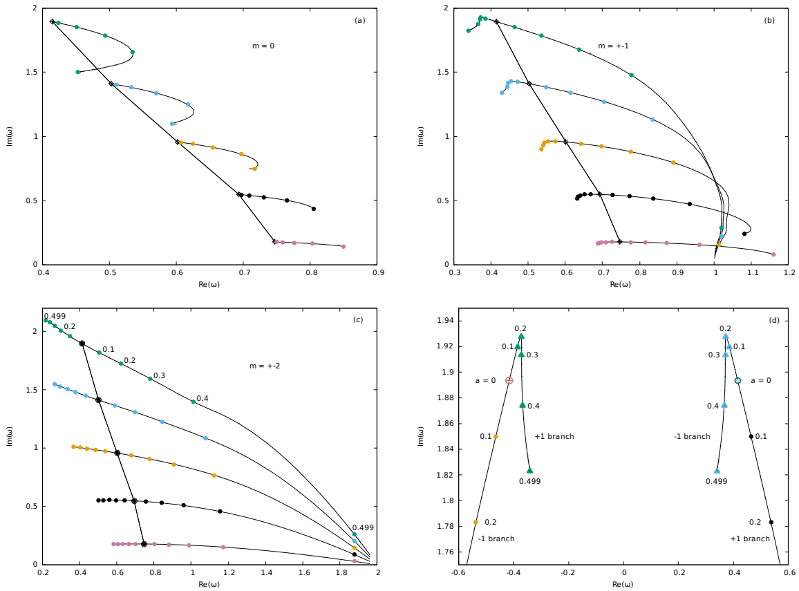
Figure 3. Five Kerr quasi-normal frequencies for l = 2 and m = 0, \pm 1 , and \pm 2 . The curves are parameterized by the value of the rotation parameter a . The broken line indicates the Schwarzschild limit of a = 0 , and the ends of each curve are near the Kerr limit with a = 0.4999 . The solid dots occur at a = 0.1, 0.2, 0.3, 0.4 , and 0.4990 . The lowermost curve in each of these plots corresponds to the curves in figure 1a of Detweiler (1980). Tables 2 and 3 list some of the frequencies plotted in (a) and (b). Part (d) is a detail of the top-most curve in (b), and illustrates the complex conjugate symmetry of the Kerr quasi-normal frequencies.
