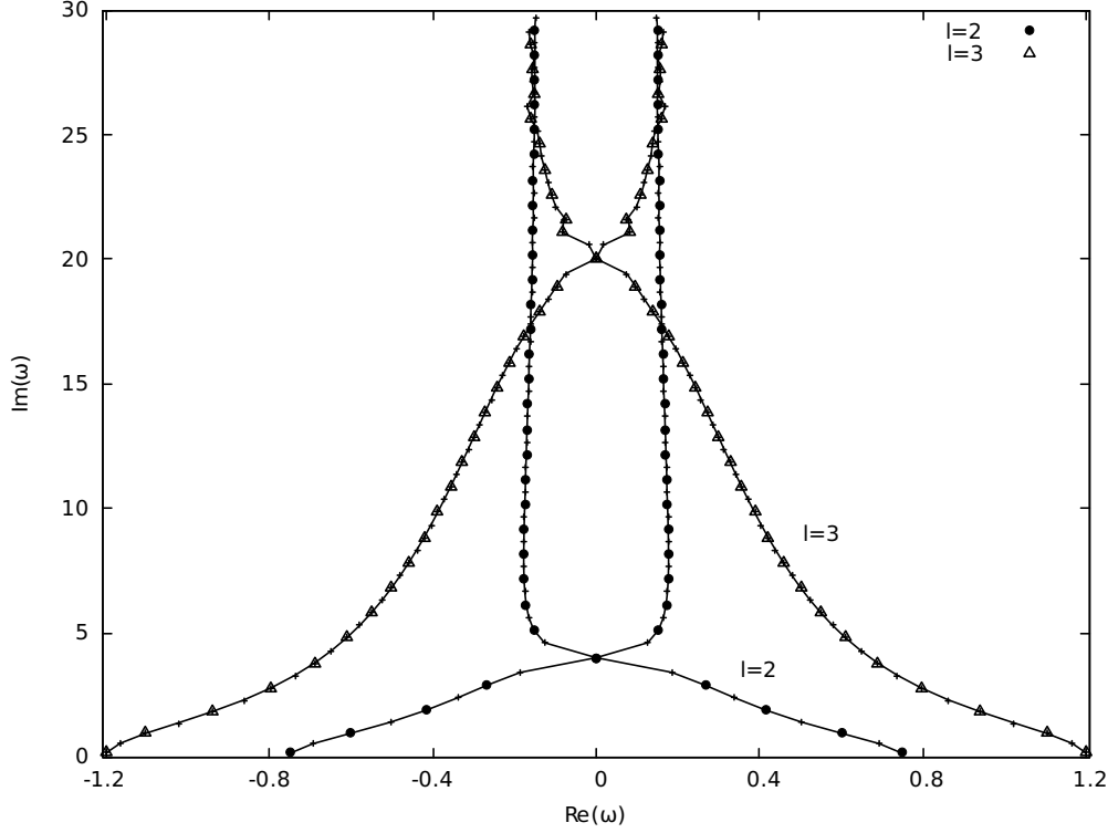
Figure 1. First 60 Schwarzschild gravitational quasi-normal frequencies for l = 2 and l = 3 . The odd order frequencies are prominently marked; a few even-order frequencies are indicated as short bars perpendicular to the curves connecting the points.
